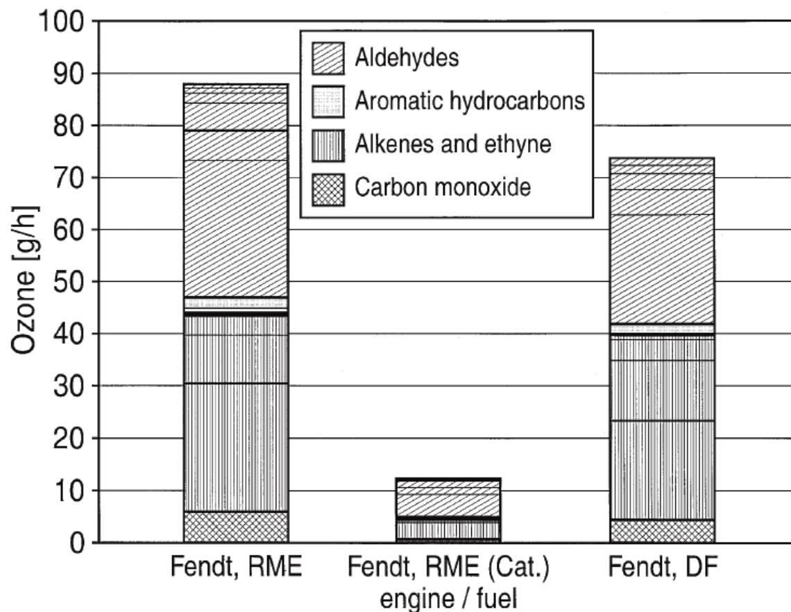
FIG. 11. Calculated ozone-forming potentials of diesel fuel and biodiesel exhaust emissions; Fendt tractor, 5-mode test. See Figure 2 for abbreviations.
